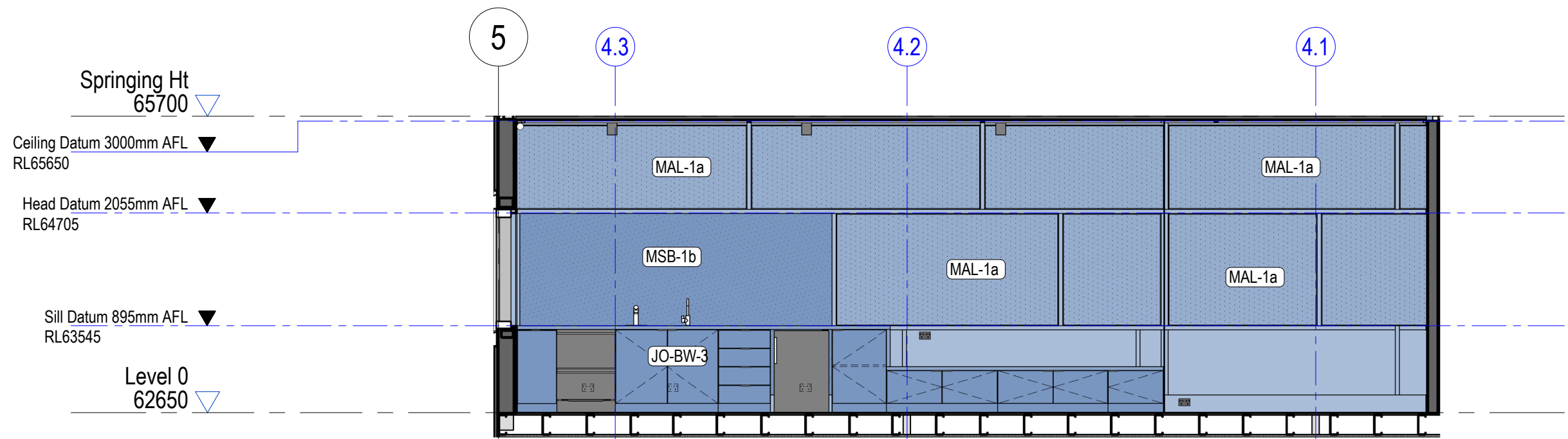
5 0.08 - Boardroom - West Elevation 1 : 50
