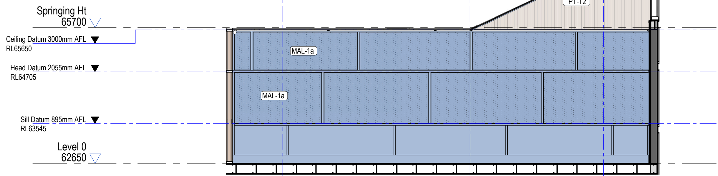
3 0.08 - Boardroom - East Elevation 1 : 50
