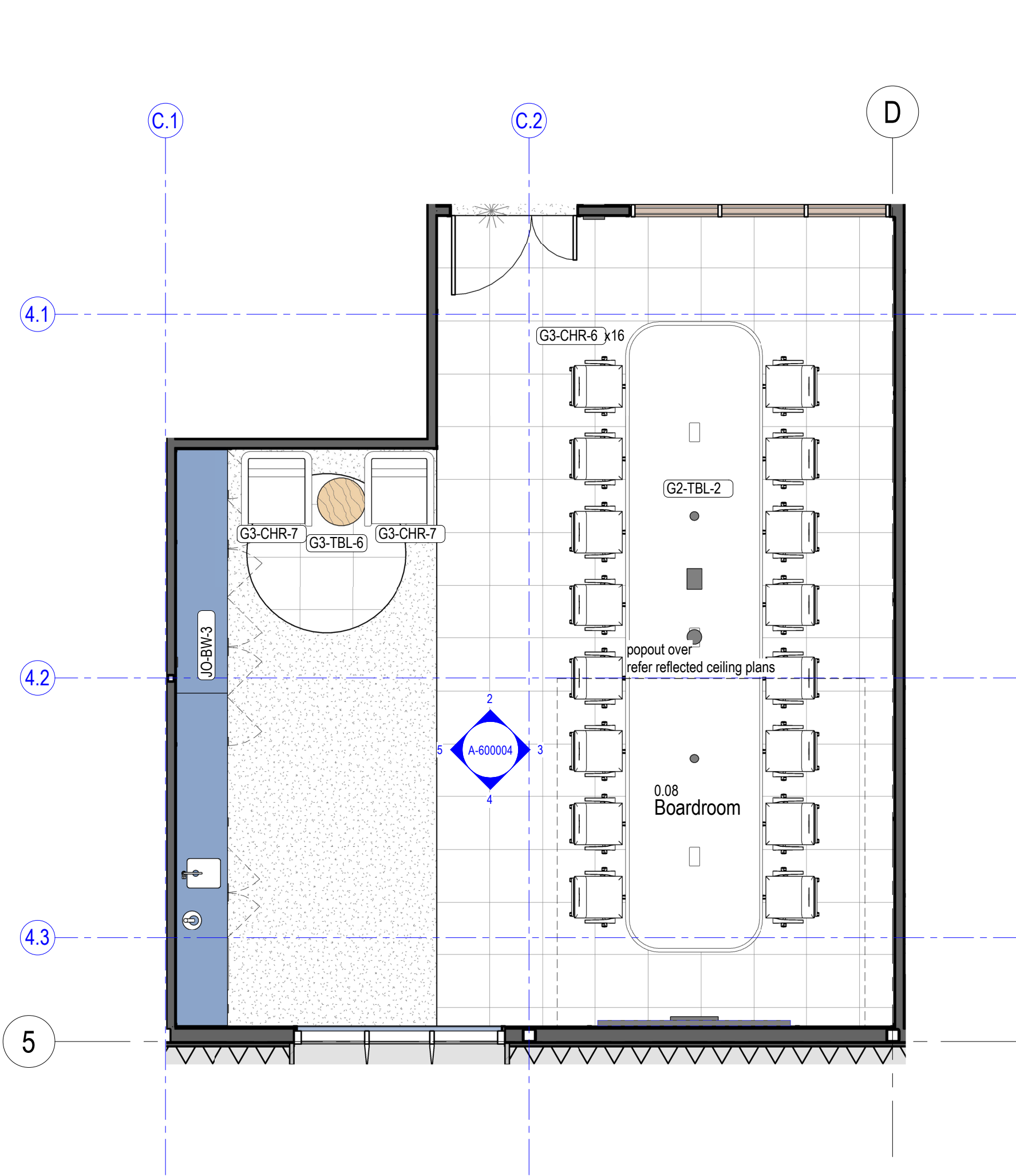
1 0.08 - Boardroom - Plan 1 : 50
