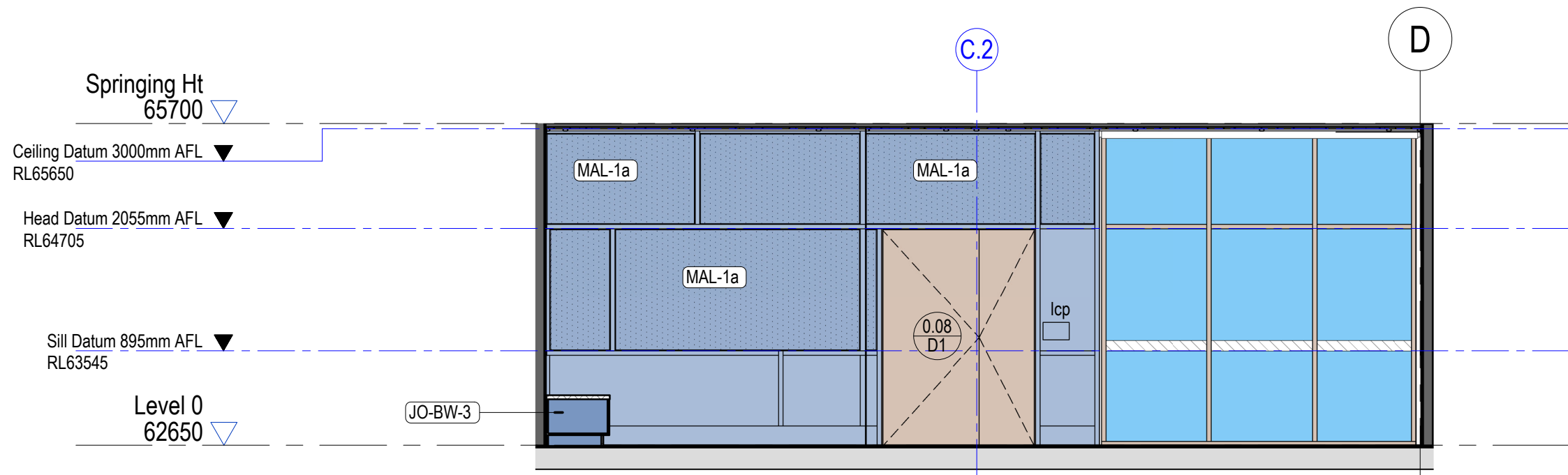
2 0.08 - Boardroom - North Elevation 1 : 50
