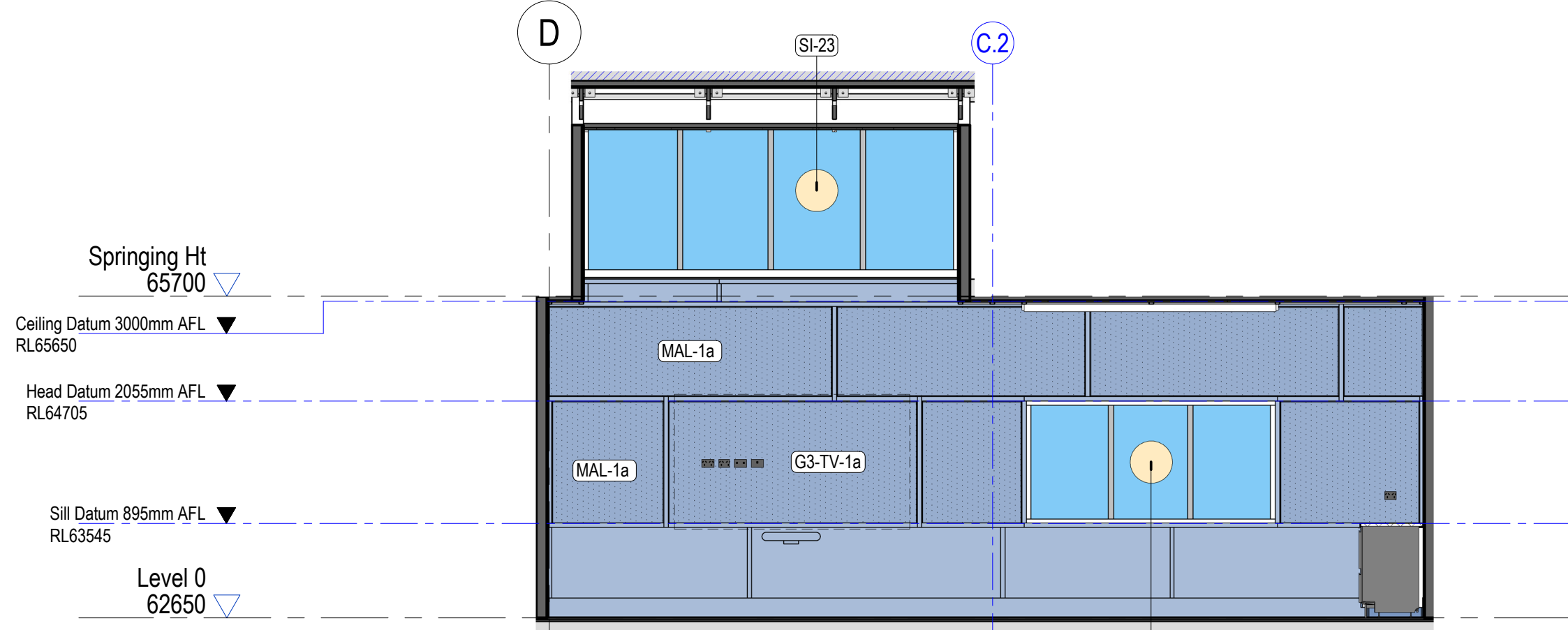
4 0.08 - Boardroom - South Elevation 1 : 50
